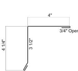
Box Gable Trim 4-1/4" Face
