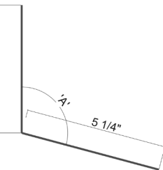
Slope Transition Flashing 5-1/4"
