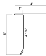
Extended Gable Trim 5" Face
