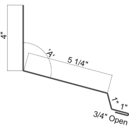
Fascia Cover 7-1/2" L-shaped
