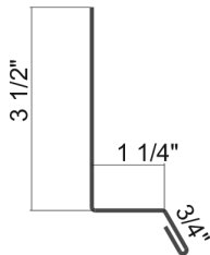
Sill Trim 1-1/4"
