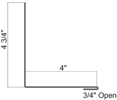
Sidewall Trim #5
