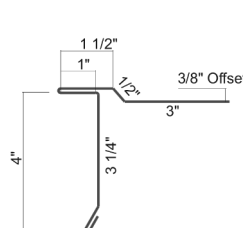
Extended Gable Trim w/Offset 4" Face
