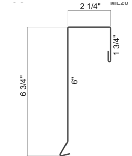
Box Gable Trim 6-3/4" Face
