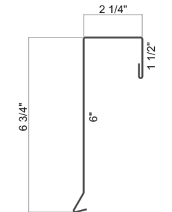
Box Gable Trim 6-3/4" Face
