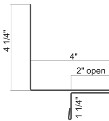
Sidewall Expansion Joint Flashing
