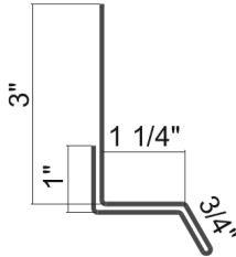
Sill Trim 1-1/4"
