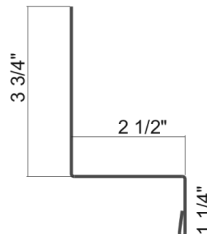
Highwall Trim 4-3/4"
