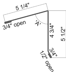
Peak Flashing 5-1/2"
