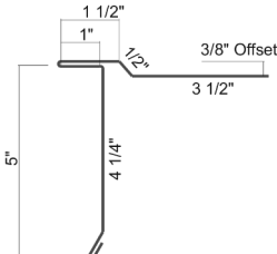
Extended Gable Trim w/Offset 5" Face
