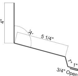
Low Wall Flashing #1
