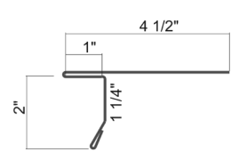
Extended Gable Trim, 2" Face
