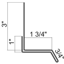
Sill Trim 1-3/4"
