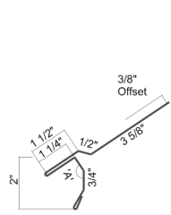
Steep Sloped Ext. Eave w/Offset 2" Face
