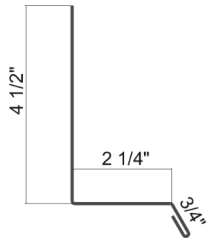
Sill Trim 2-1/4"
