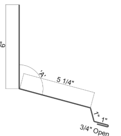
Low Wall Flashing #2
