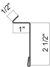
Reglet Flashing 2-1/2"
