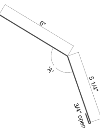
Gambrel Flashing
