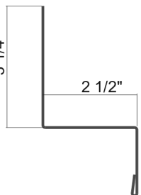
Vented Highwall Trim 4"
