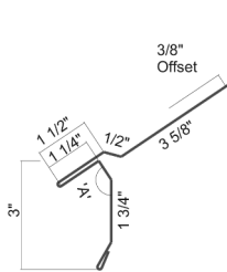
Steep Sloped Ext. Eave w/Offset 3" Face
