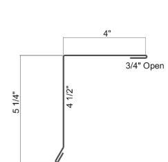
Box Gable Trim 5-1/4" Face
