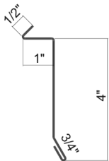
Reglet Flashing 4"
