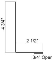
Sidewall Trim #6
