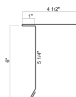
Extended Gable Trim 6" Face
