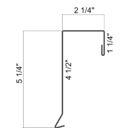
Box Gable Trim 5-1/4" Face
