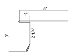
Extended Gable Trim 3" Face
