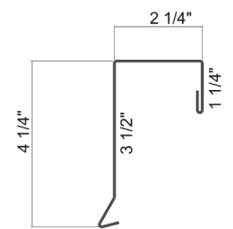
Box Gable Trim 4-1/4" Face
