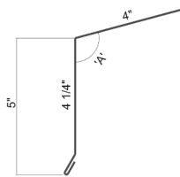
Extended Gable Trim 4" Face
