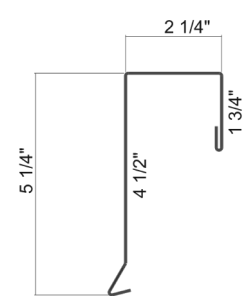
Box Gable Trim 5-1/4" Face
