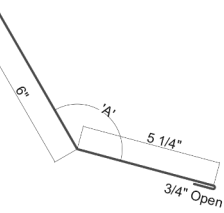
Slope Transition Flashing 5-1/4"
