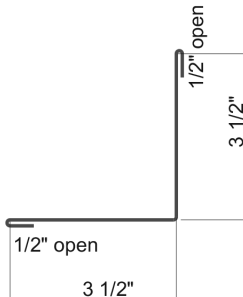
Inside Corner
