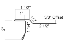
Extended Gable Trim w/Offset 2" Face
