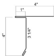
Extended Gable Trim 4" Face
