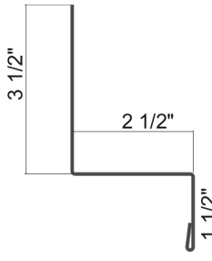
Highwall Trim 6"
