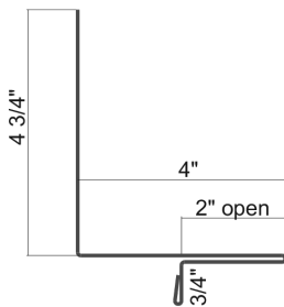
Sidewall Expansion Joint Flashing
