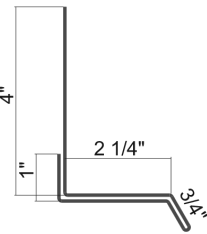
Sill Trim 2-1/4"
