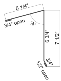
Peak Flashing 7-1/2"
