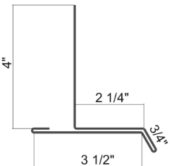
Sill Trim 2-1/4"
