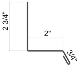
Sill Trim 2"
