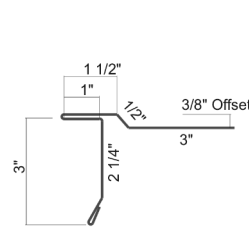
Extended Gable Trim w/Offset 3" Face
