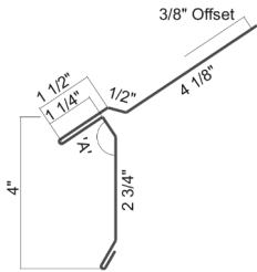
Steep Sloped Ext. Eave w/Offset 4" Face
