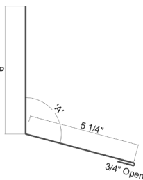
Fascia Cover 6" L-shaped
