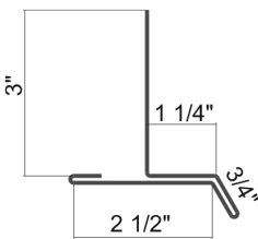
Sill Trim 1-1/4"
