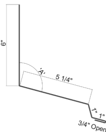
Fascia Cover 11-1/2" w/ kickout
