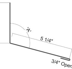
Vented Highwall Trim 6"
