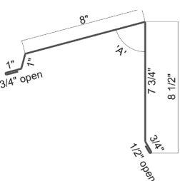
Vented Peak Flashing
