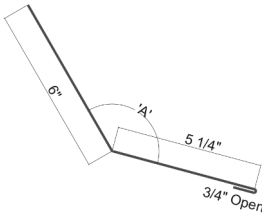
Fascia Cover 9" L-shaped
