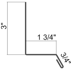
Sill Trim 1-3/4"
