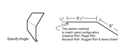
Notched Upper Gambrel Flashing
