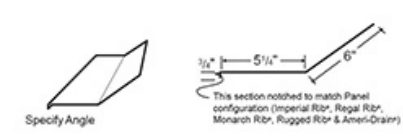
Notched Lower Gambrel Flashing
