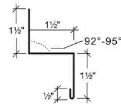
'PBR' Stack Joint Trim
